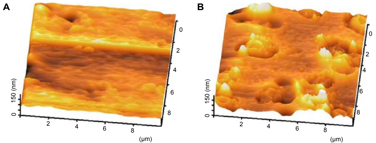
Figure 9 Representative 3D topographical view of control and 24 hours coated sample obtained by AFM. Notes: (A) Pristine mPE, (B) A-24 h-mPE. Abbreviations: mPE, metallocene polyethylene; AFM, atomic force microscopy; D, dimensional; A-12 h-mPE, 12 hours Aloe vera -coated; A-24 h-mPE, 24 hours Aloe vera -coated.
