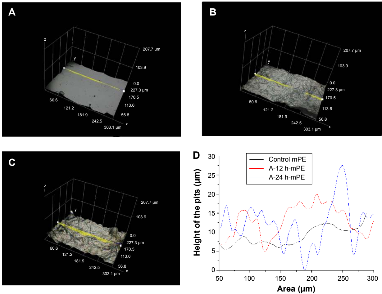
Figure 8 Hirox 3D images of control and extract-coated mPE samples taken at 1,000× with profiles. Notes: (A) Pristine mPE, (B) A-12 h-mPE, (C) A-24 h-mPE, (D) outline of crests and troughs in figure (8A, B and C). Abbreviations: mPE, metallocene polyethylene; D, dimensional; A-12 h-mPE, 12 hours Aloe vera -coated; A-24 h-mPE, 24 hours Aloe vera -coated.
