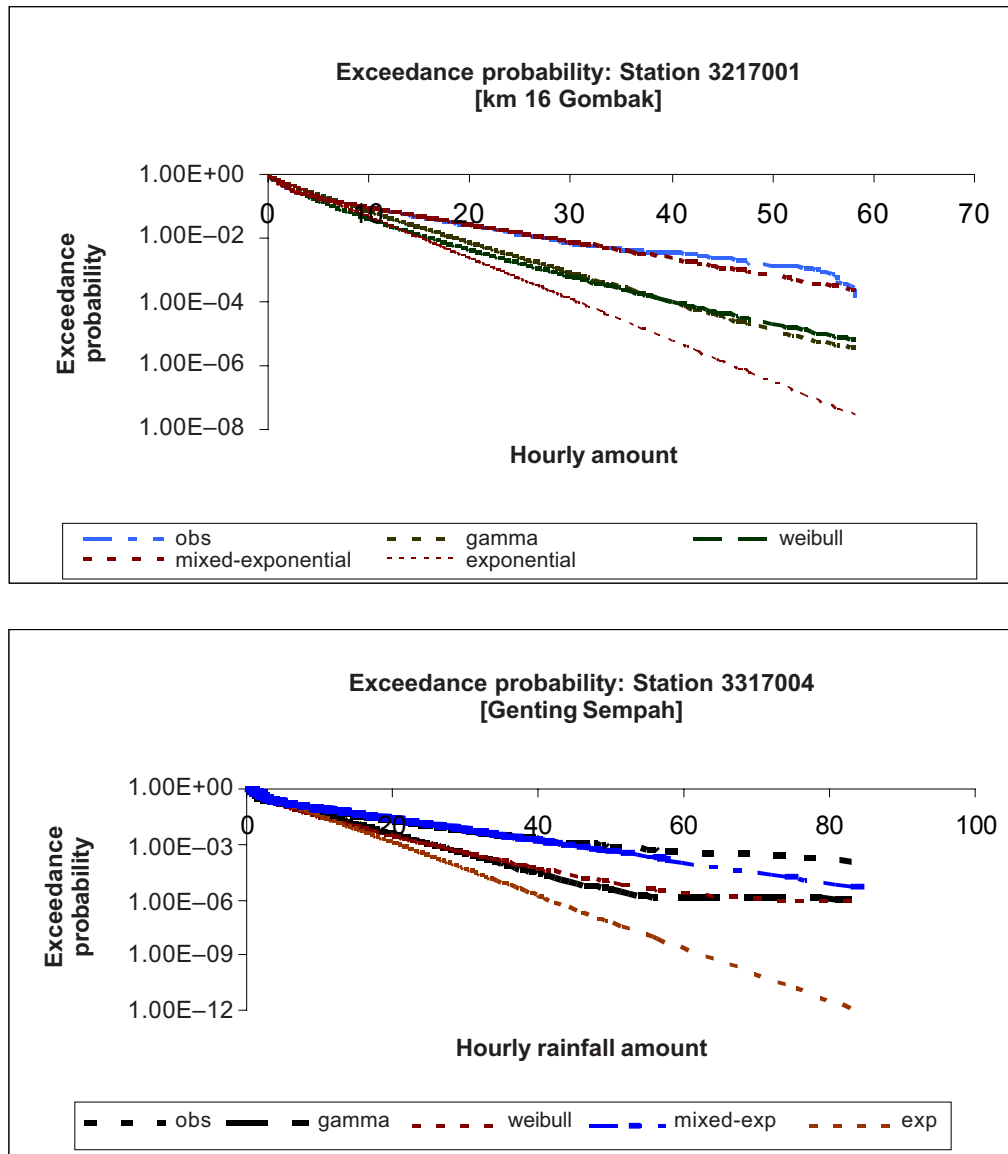
Figure 1 Exceedance probability for Stations 3217001 and 3317004
