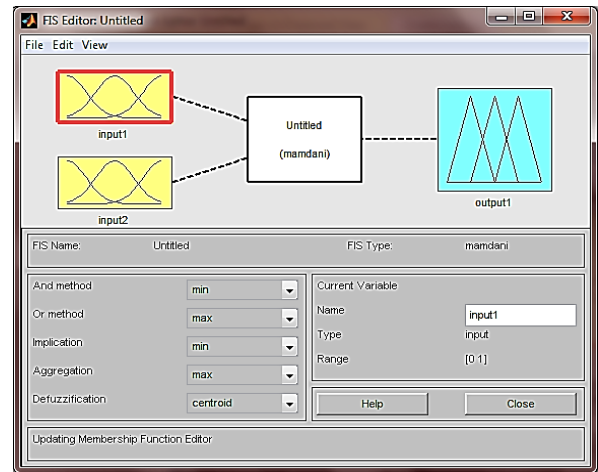
Figure 12 FIS Editor
