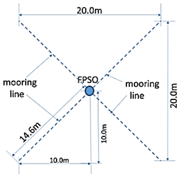
Figure 3 Arrangement of mooring lines and anchor in wave basin
