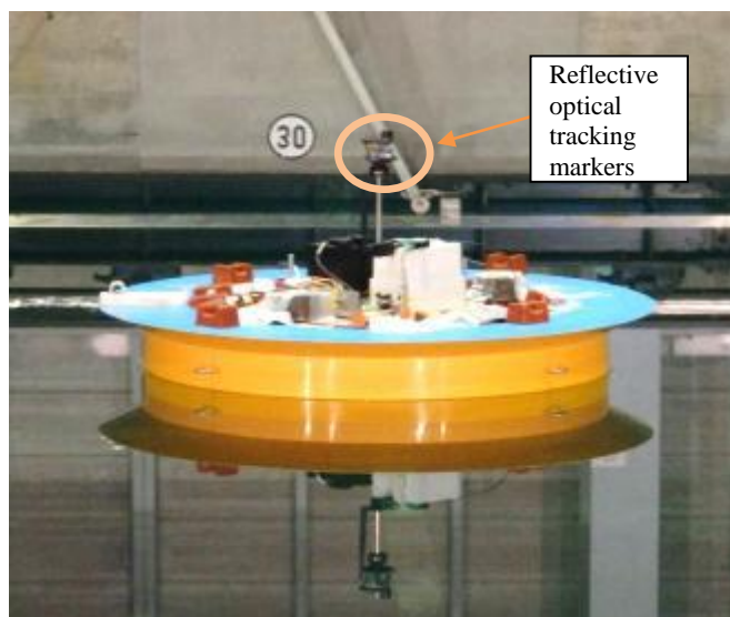
Figure 4 FPSO model fixed with mooring lines in wave basin in static condition
