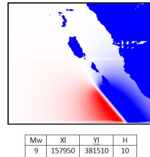
Figure 1 Tsunami source zone model at Pagai megathrust block
