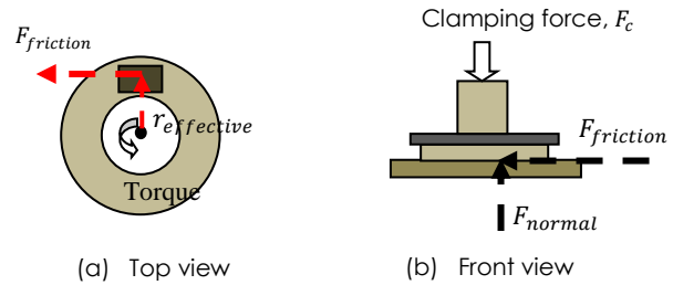
Figure 9 Brake torque model in contact interface [13]
