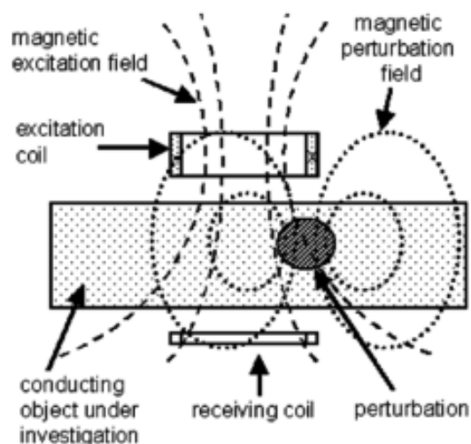
Figure 7 Principle of magnetic induction spectroscopy 20
