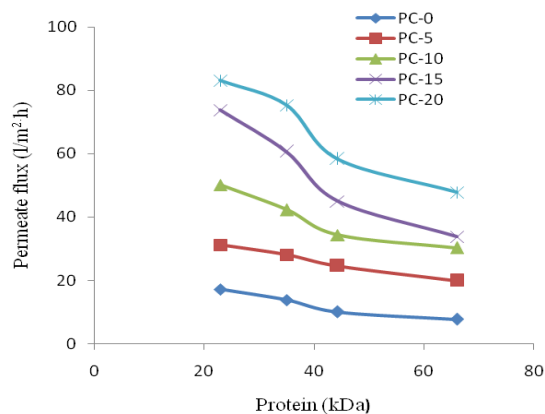
Figure 1 Permeate fluxes of different molecular weight of proteins for PSf and PSf/CAP blend membranes at operating pressure of 3 bar
