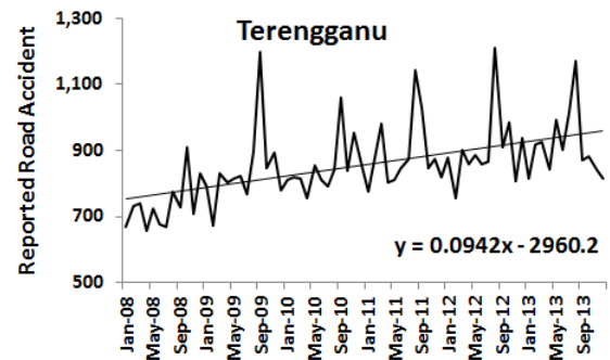
Figure 3 The process of de-trending monthly total registered accident in Terengganu
