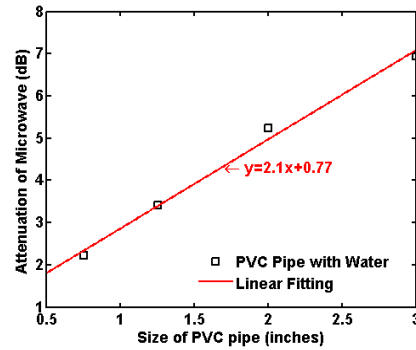
Figure 8 Graph of attenuation of microwave against size of PVC pipe with water
