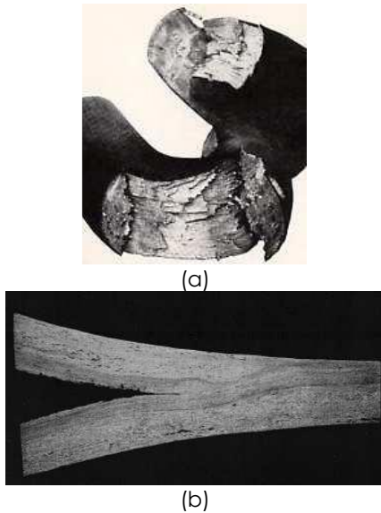
Figure 3 Examples of wrought iron [17]
