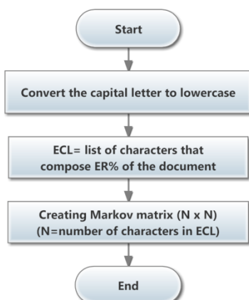
Figure 2 Pre-processing and ECL extraction
