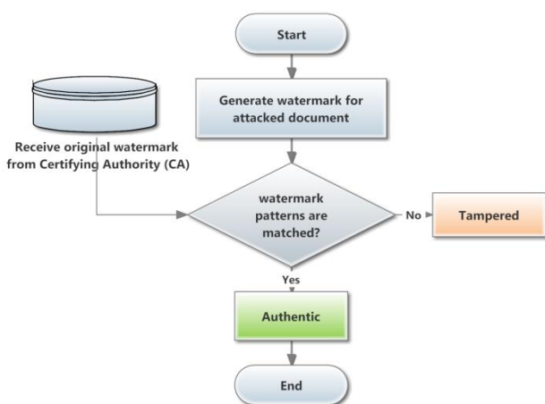
Figure 3 Watermark extraction and detection
