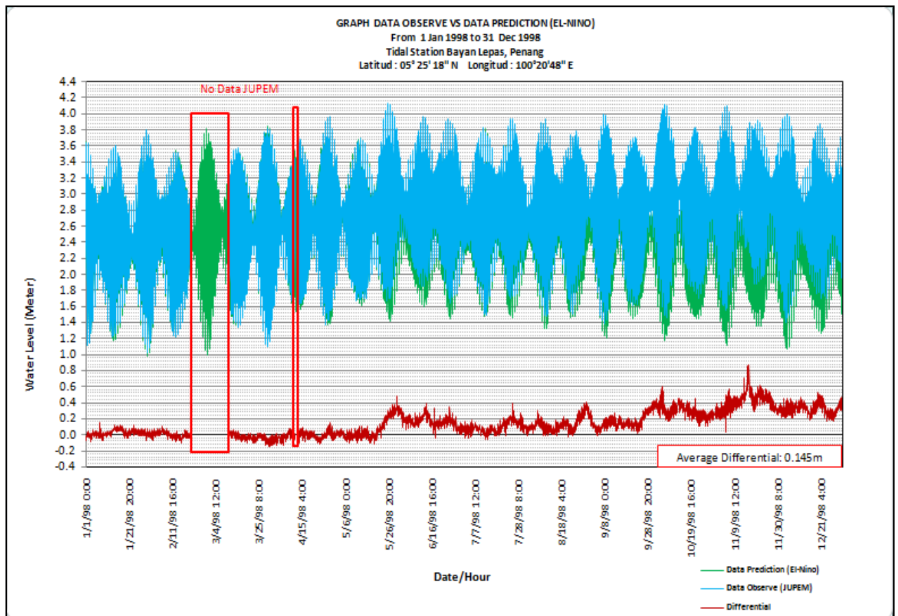
Figure 2 Differential graph for tidal observation and tidal prediction at Bayan Lepas, Penang during El Nino effect
