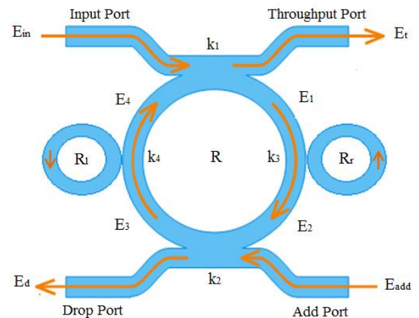
Figure 1 Panda ring resonator configuration consisting add-drop multiplexer and nano-ring on both sides
