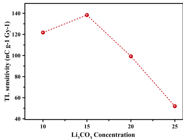
Figure 4 TL sensitivity versus Li 2 CO 3 concentration of the prepared glass samples
