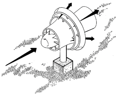
Figure 19 Free-flow turbine [21]
