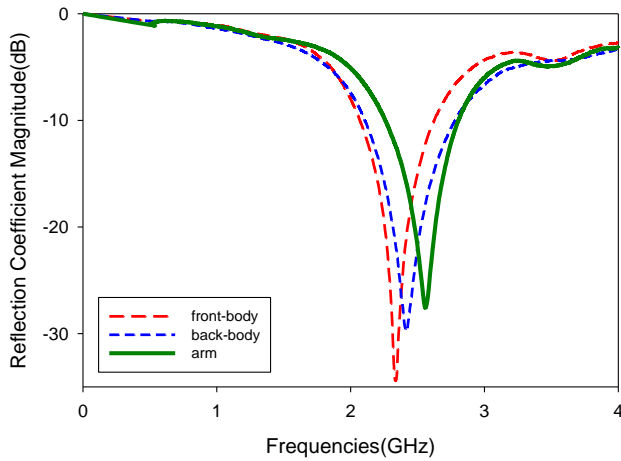
Figure 12 Shield It Fabric antenna On-Body Measurement
