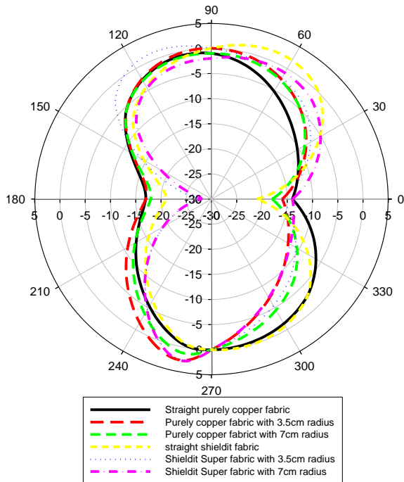
Figure 6 E-Plane
