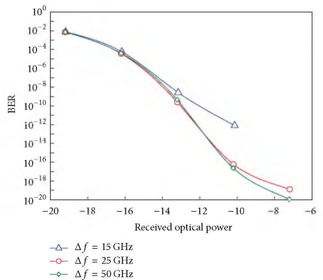
FIGURE 8: The system performance at different wavelength inter-leaves.
