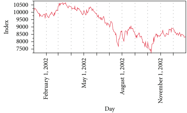
FIGURE 2: Unprocessed data for year 2002 of DJI.
