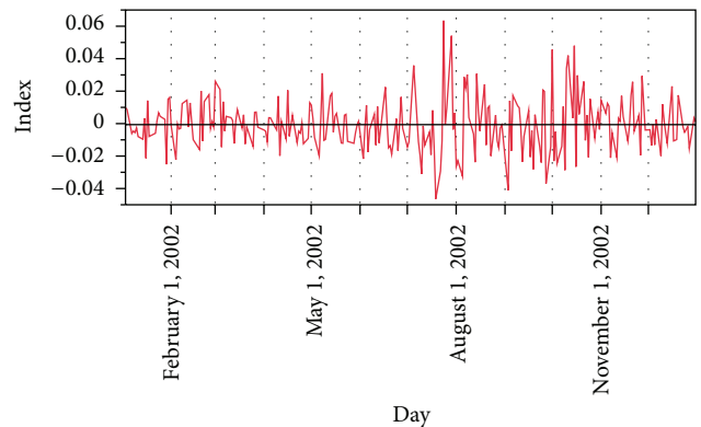
FIGURE 3: Processed data for year 2002 of DJI.
