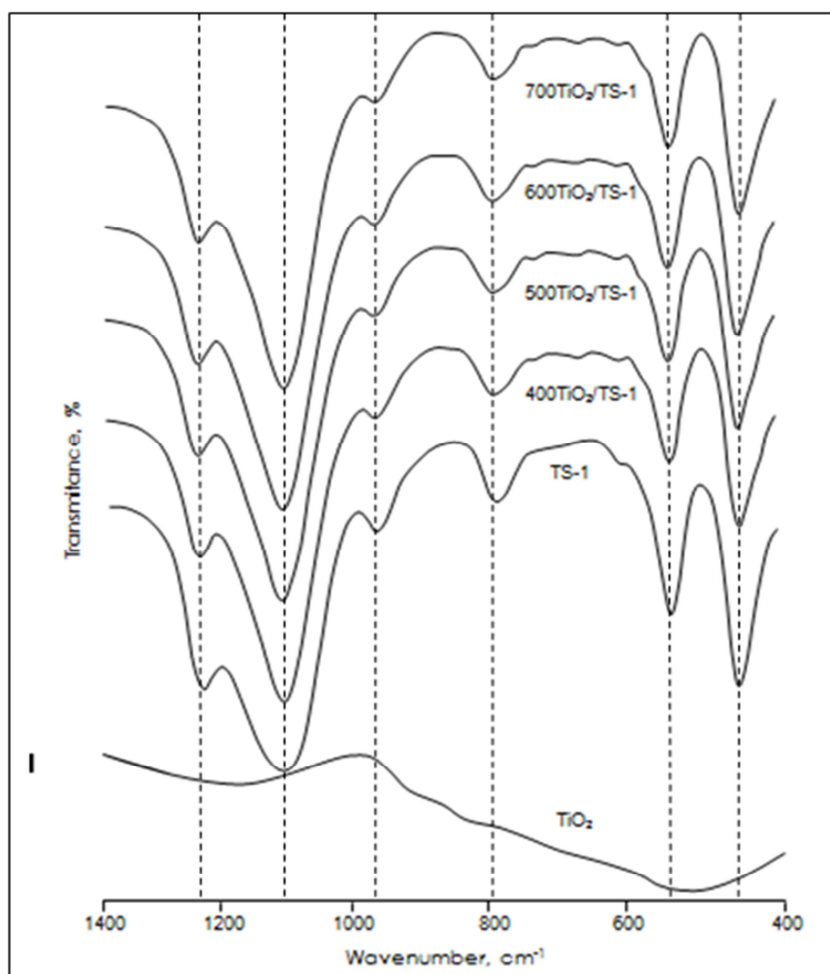
Figure 2 Framework infrared spectra of TiO 2 , TS-1 and TiO 2 /TS-1 calcined at different temperatures (400, 500, 600 and 700°C) for 3 h.
