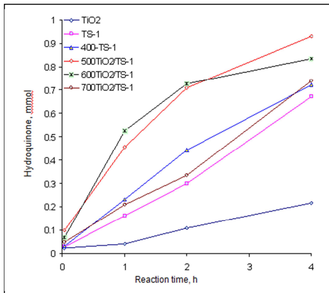
Figure 6 Catalytic performance of TiO 2 , TS-1, and TiO 2 /TS-1 catalysts for hydroquinone production from phenol hydroxylation reaction with H 2 O 2 at 70°C.
