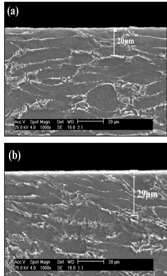
Figure 5 SEM micrographs of the cross-sectional sub-surface of the milled alloy at feed rate of 0.03 m/min and cutting speed of 200 m/min using and using (a) new tool and (b) worn tool
