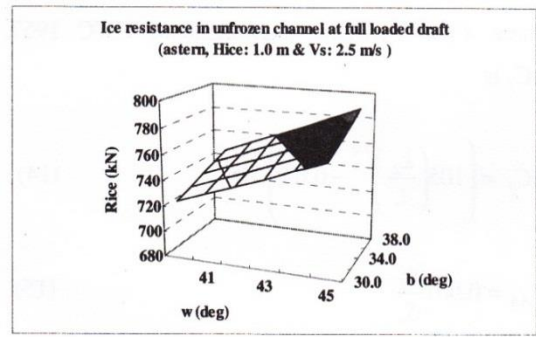
Figure 11 Ice resistance in unfrozen channel at full loaded draft, astern without propeller, H-ice: 1.0 m and Vs: 2.5 m/s
