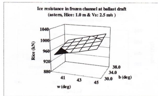
Figure 14 Ice resistance in frozen channel at ballast draft, astern without propeller, H-ice: 1.0 m and Vs: 2.5 m/s
