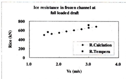
Figure 17 Comparison ice resistance of selected hull form in frozen channel at full loaded draft in astern with existing DAT “Tempera” (4)
