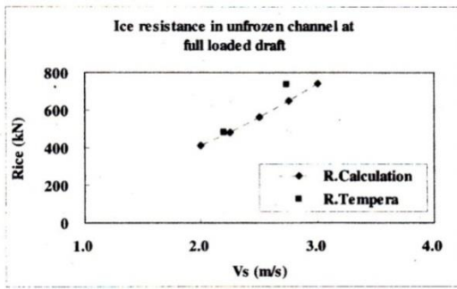
Figure 15 Comparison ice resistance of selected hull form in unfrozen channel at full loaded draft in astern with existing DAT “Tempera” 4
