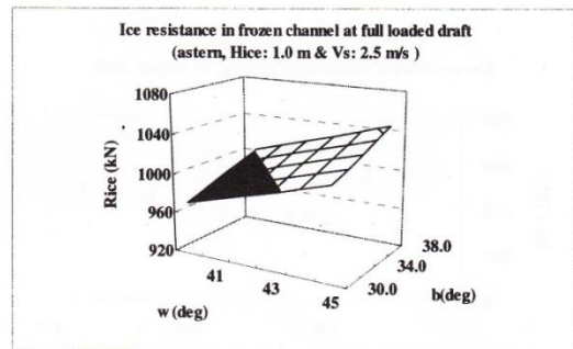
Figure 13 Ice resistance in frozen channel at full loaded draft, astern without propeller, H-ice: 1.0 m and Vs: 2.5 m/s
