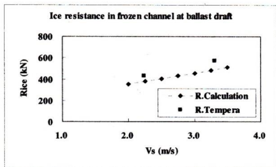
Figure 18 Ice resistance in frozen channel at ballast draft astern with propeller and then compare with existing DAT “Tempera” 4
