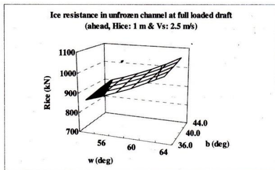
Figure 9 Ice resistance in frozen channel at full loaded draft, ahead, H-ice: 1.0 m and Vs: 2.5 m/s
