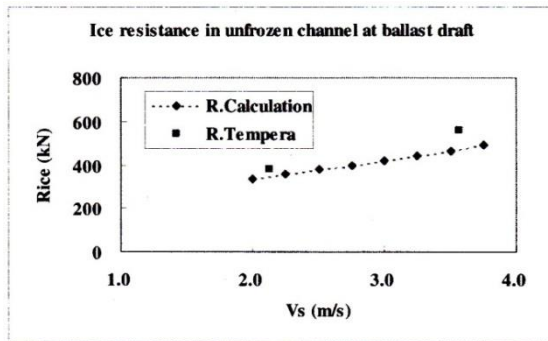
Figure 16 Comparison ice resistance of selected hull form in unfrozen channel at ballast draft in astern with existing DAT “Tempera” 4
