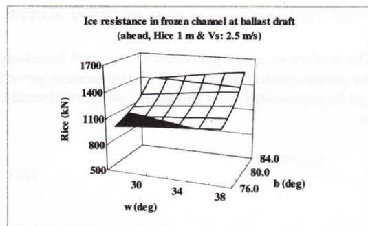
Figure 10 Ice resistance in frozen channel at ballast draft, ahead, H-ice: 1.0 m and Vs: 2.5 m/s
