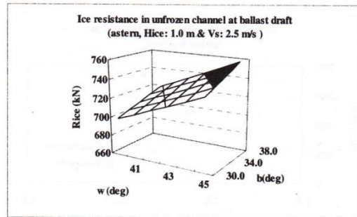
Figure 12 Ice resistance in unfrozen channel at ballast draft, astern without propeller, H-ice: 1.0 m and Vs: 2.5 m/s
