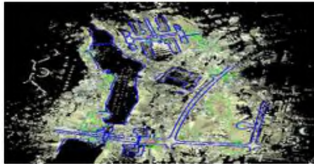
Figure 4. Digitizing of topographic features in Cyclone II Topo (blue cloud).
