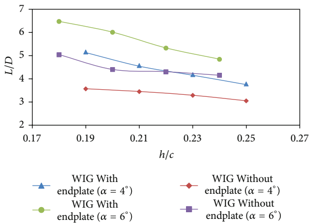
FIGURE 8: Lift-to-drag ratio ( L/D ) of WIG craft model with and without endplates versus ground clearance ( h/c ) at different angles of attack.
