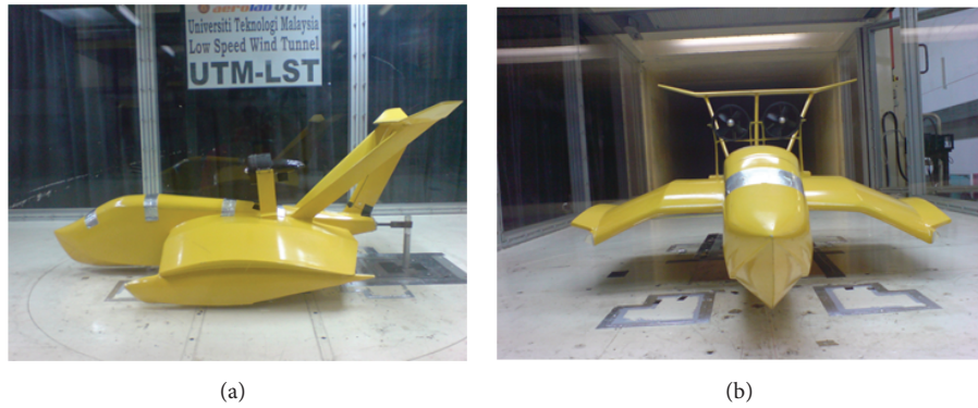
FIGURE 4: Wind tunnel test for WIG craft model: (a) model with endplates and (b) model without endplates.
