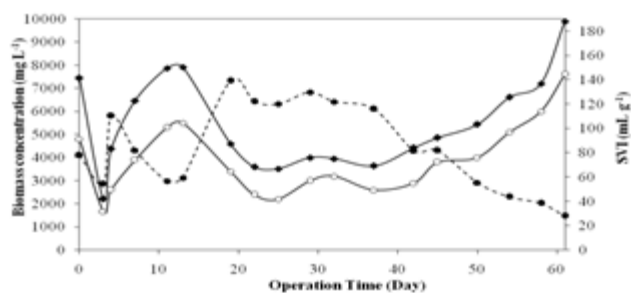
Figure 3 The concentration of biomass and SVI during granulation process (●) MLSS concentration; (○) MLVSS concentration; (●) SVI.
