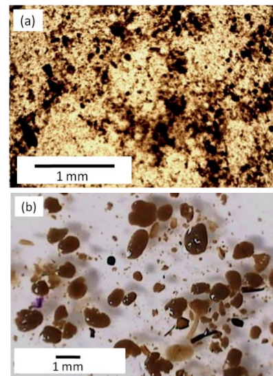
Figure 1 Morphology of AGS in the reactor (a) Fluffy and filamentous aerobic granular sludge at 14 th day of inoculation (b) Matured and dense aerobic granular sludge at day 60 of inoculation
