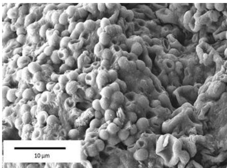
Figure 2 SEM observation of surface microstructure of matured aerobic granules and coccoid bacteria densely packed at the outer layer of granule
