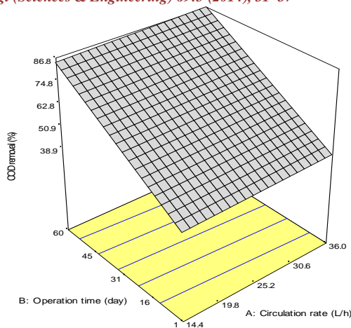
Figure 5 Effect of circulation rate and operation time on COD removal
