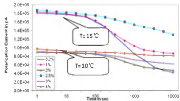
Fig. 3. Effect of paper moisture content on the polarization current, measured at 15°C and 10°C [13].
