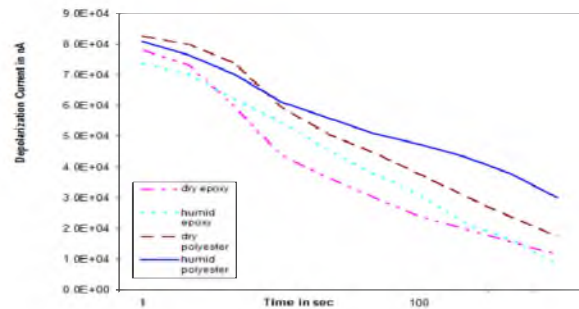
Fig. 8. Discharge currents for epoxy-mica bars and a polyester-mica coil, before (dry) and after (humid), one week under a humid atmosphere [6].
