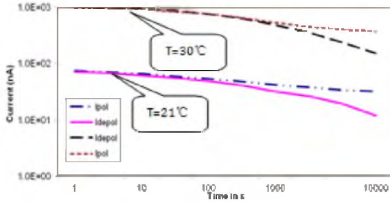
Fig. 9. Polarization and depolarization current of 2 km XLPE cable, after 4 years in service (T=21 °C), and 5 years later, after supplying fault current (T=30°C) [4].
