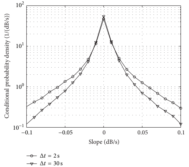
FIGURE 6: Conditional distribution of fade slope for \Delta t = 2 s and \Delta t = 30 s at A = 1 dB.
