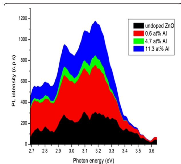
Figure 12 PL spectra of the as-synthesized ZnO:Al nanowires on silicon substrate showing intensity versus energy.
