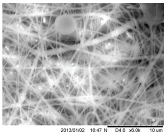
FIGURE 5: SEM image 8 wt% PCL/7% alkali treated chitosan (50/50).
