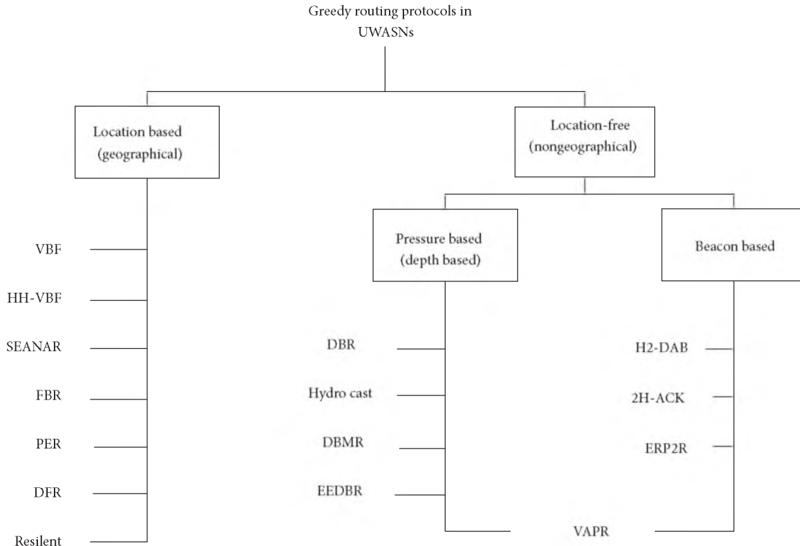
FIGURE 2: Taxonomy of greedy routing protocols in UWASNs.
