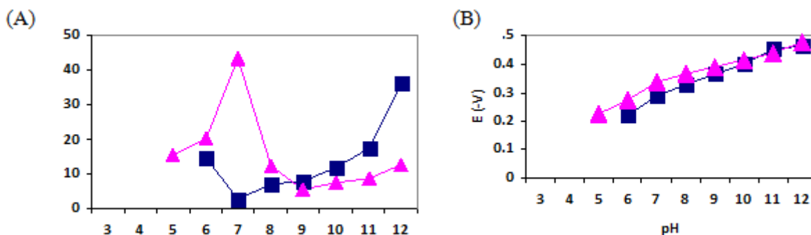
Figure 3. The peak current (A) and peak potential (B) versus pH of BRB for ampicillin (▲) and penicillin G (■), E_i = 0 V, E_{acc} = 0 V, t_{acc} = 30 s, scan rate = 0.02 Vs -1 . Concentrations of ampicillin and penicillin G were 5 \times 10^{-7} mol/L.
