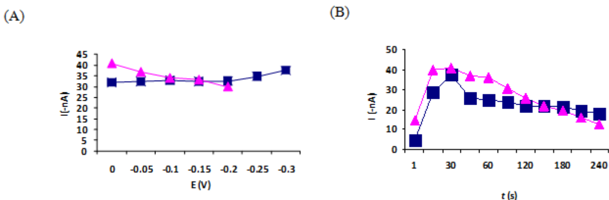
Figure 4. The effect of (A) initial potential and (B) accumulation time in 0.04 mol/L BRB on ampicillin (▲) and penicillin G (■) reduction peak at optimum pH. E_{acc}=0 V, t_{acc}=30 s, scan rate = 0.02 \text{Vs}^{-1} . Concentration of ampicillin and penicillin G were 5 \times 10^{-7} mol/L.
