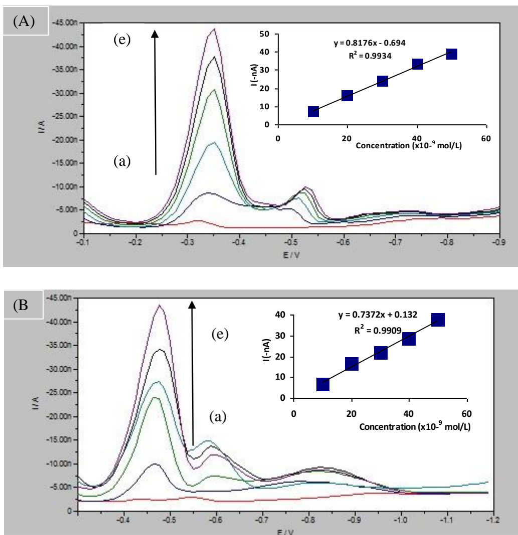
Figure 5. DPCSV at HMDE calibration for (A) ampicillin and (B) penicillin B in concentration of 1.0 - 5.0 × 10 -8 mol/L in 0.04 mol/L BRB solution at pH 7 and pH 12 with optimum conditions for each drugs and with scan rate = 0.02 Vs -1 .
