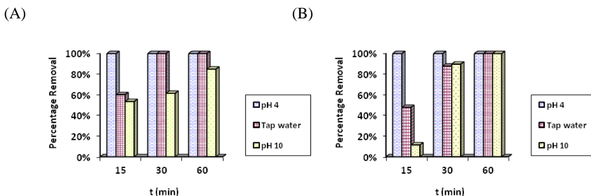
Figure 6. The degree of degradation (%) of ampicillin versus treatment time in three different media using (A) Ru-Ir-TiO 2 (20:30:50) and (B) Ru-Ir-TiO 2 (40:10:50) anode.
