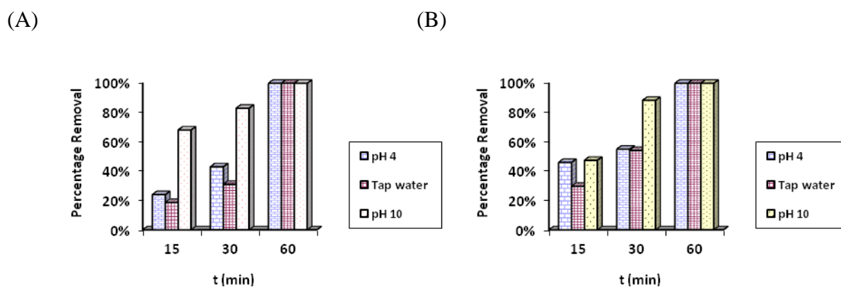
Figure 7. The degree of degradation of penicillin G (%) versus treatment time in three different media using (A) Ru-Ir-TiO 2 (20:30:50) and (B) Ru-Ir-TiO 2 (40:10:50) anode
