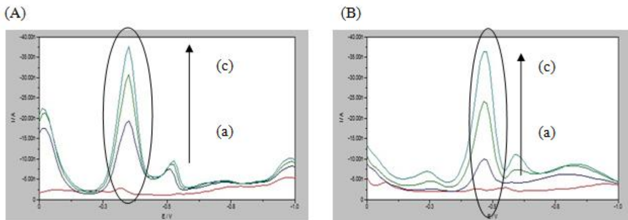
Figure 1. DPCS voltammograms at HMDE in 0.04 mol/L BRB for (A) ampicillin at pH 7 (B) penicillin G at pH 12, E_i = 0 V, E_{acc} = 0 V, t_{acc} = 30 s, scan rate = 0.02 Vs -1 ; (a) 1 \times 10^{-7} mol/L (b) 3 \times 10^{-7} mol/L (c) 5 \times 10^{-7} mol/L
