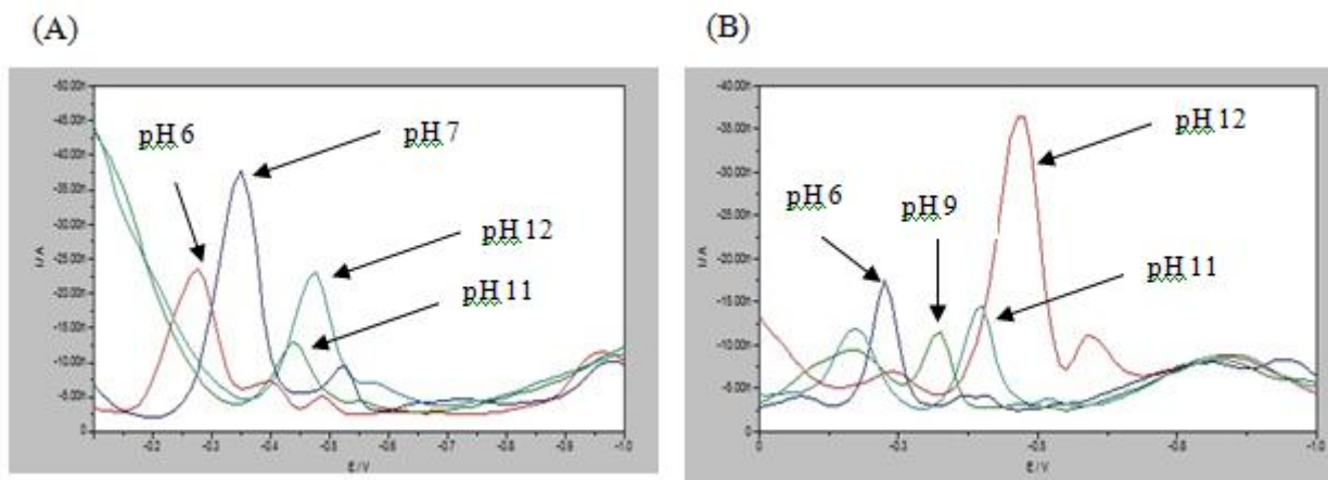
Figure 2. DPCS voltammograms at HMDE in 0.04 mol/L BRB for (A) ampicillin (B) penicillin G at various pH, E_i = 0 V, E_{acc} = 0 V, t_{acc} = 30 s, scan rate = 0.02 Vs -1 ; concentration of ampicillin and penicillin G = 5 \times 10^{-7} mol/L.
