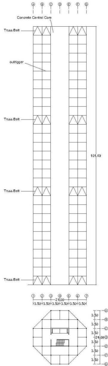
Figure 1.2 Individual building block type B
