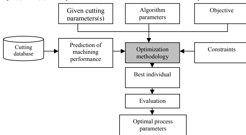
Fig. 1. PSO framework for process parameters optimization.[5]
