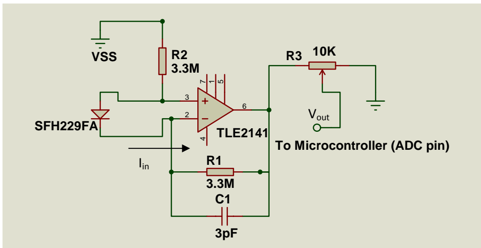
Figure 2 Receiver circuit
