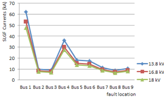
Figure. 11 . The influence of voltage level of Generator-1 for various buses as fault location at Yn-Yn transformer connection
