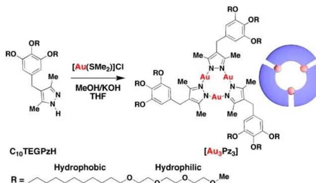
Scheme 1: Synthesis and molecular structure of [\text{Au}_3\text{Pz}_3] .
