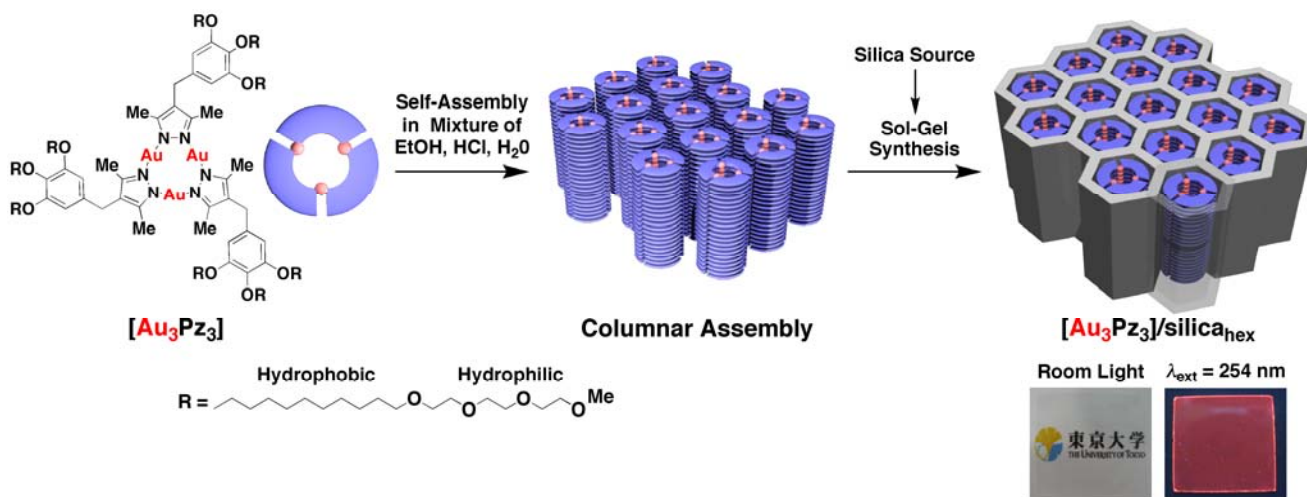
Figure 1: Schematic representation of fabrication of mesoporous silica film nanocomposite [\text{Au}_3\text{Pz}_3]/\text{silica}_{\text{hex}} with a hexagonal geometry, templated by columnar assembly of [\text{Au}_3\text{Pz}_3] via sol-gel synthesis. Photographs were taken at room temperature under room light and on exposure to ultraviolet light at 254 nm.
