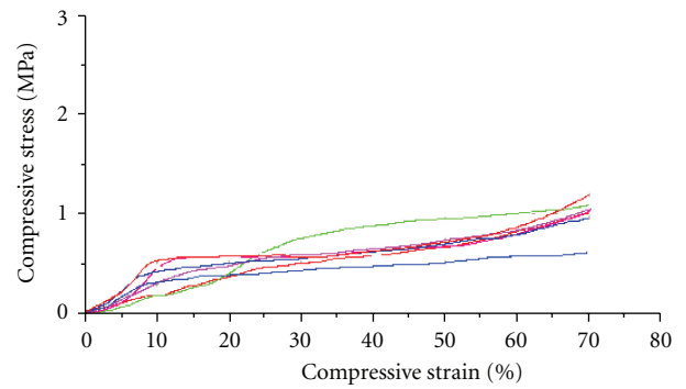
FIGURE 1: Typical compressive curves of the scaffold specimens cut from one scaffolds fabricated from combination of run 3 of Table 3.
