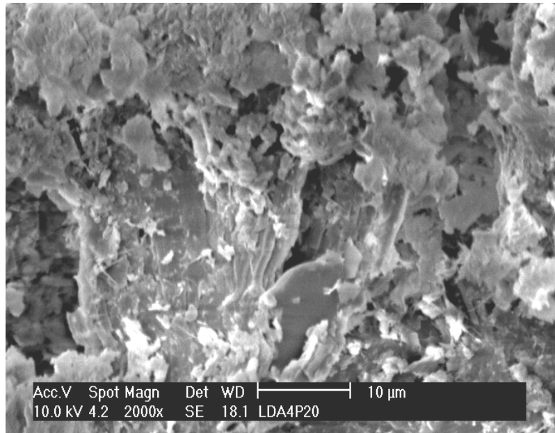
Figure 6: Photomicrograph of LDA4% with 20%FM cured for 28 days.
