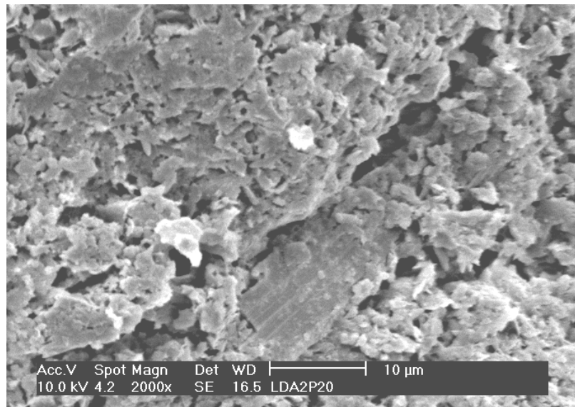
Figure 5: Photomicrograph of LDA2% with 20%FM cured for 28 days.
