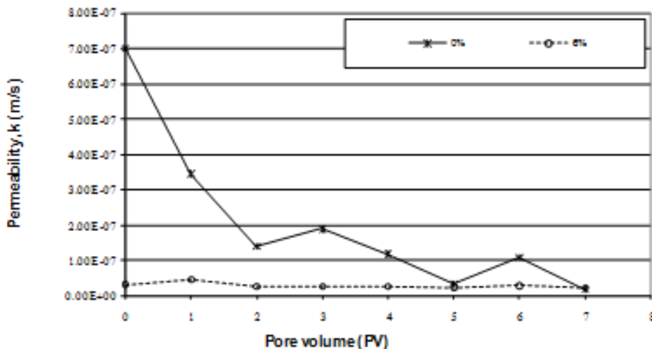
Figure 10: Permeability of unstabilised and stabilised LDA samples with leaching of water.
