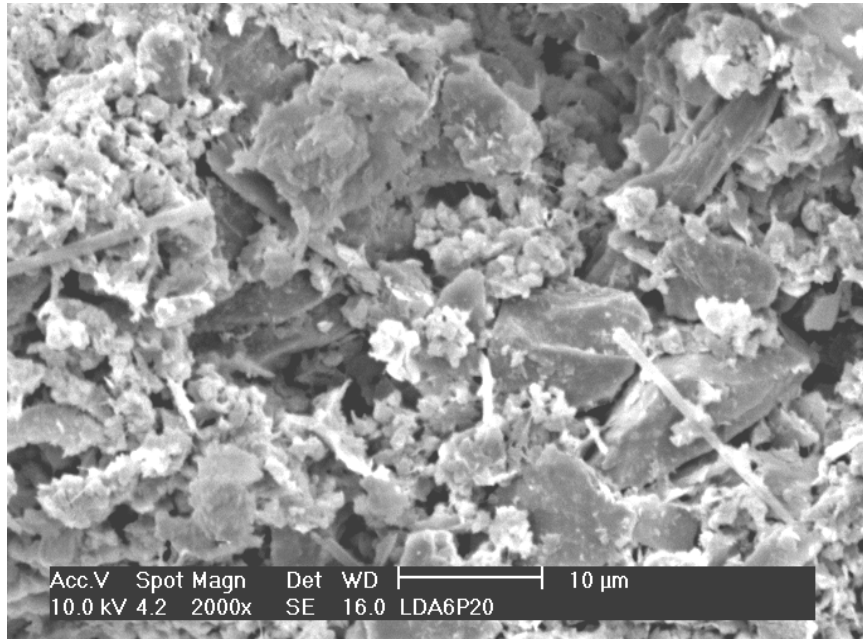
Figure 7: Photomicrograph of LDA6% with 20%FM cured 28 day.
