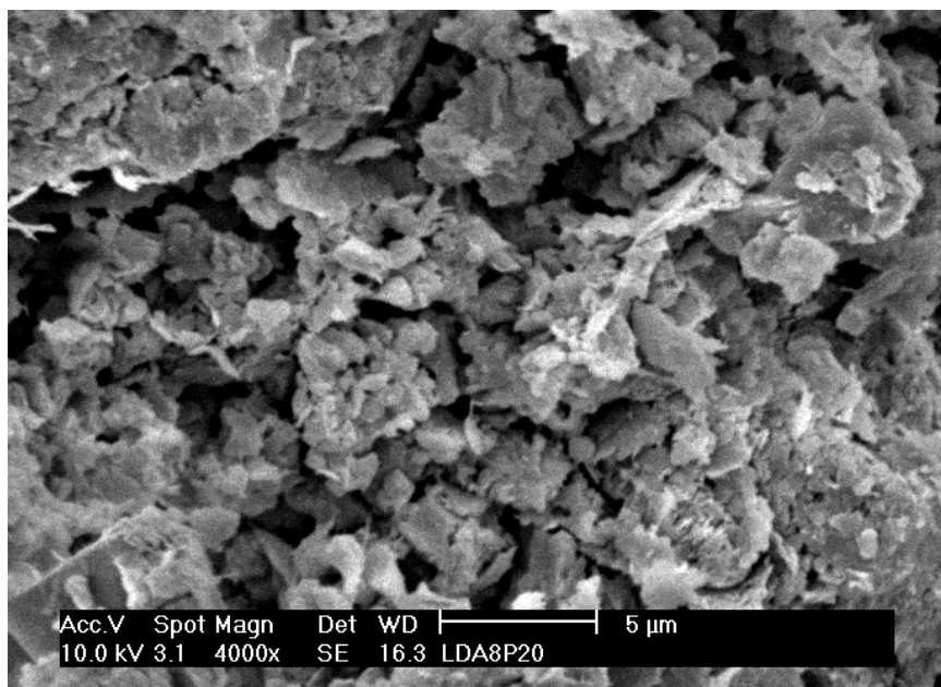
Figure9: Photomicrograph of LDA8% with 20%FM cured for 28 days.
