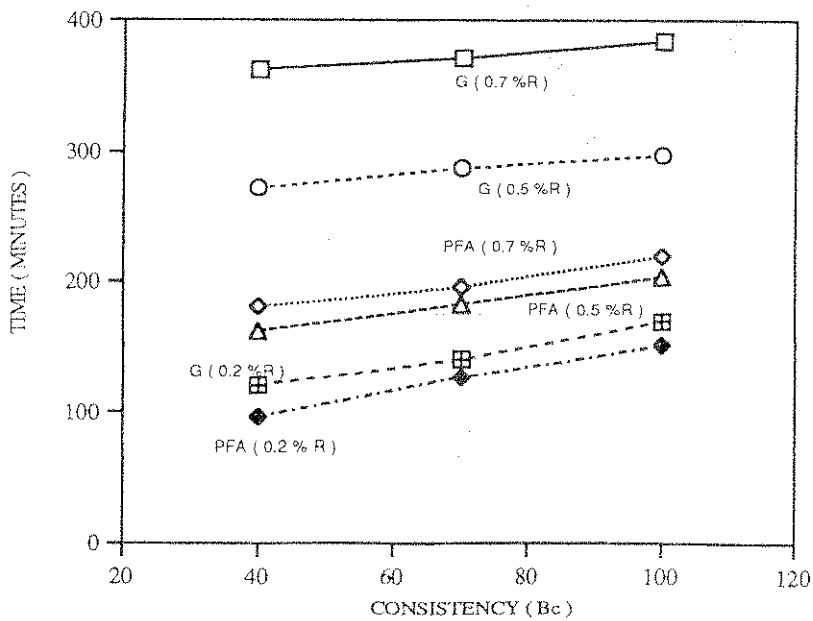
FIGURE 2. Thickening Time Profile When Cement Is Added With Different Percentage of Retarder.
