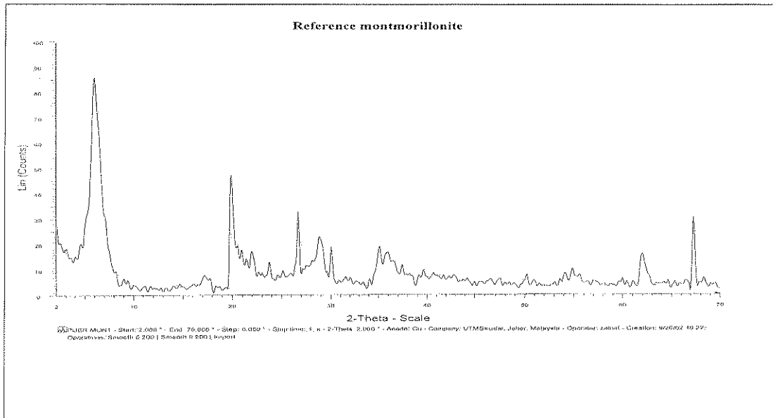
Figure 3. XRD pattern for Reference bentonite Sample
