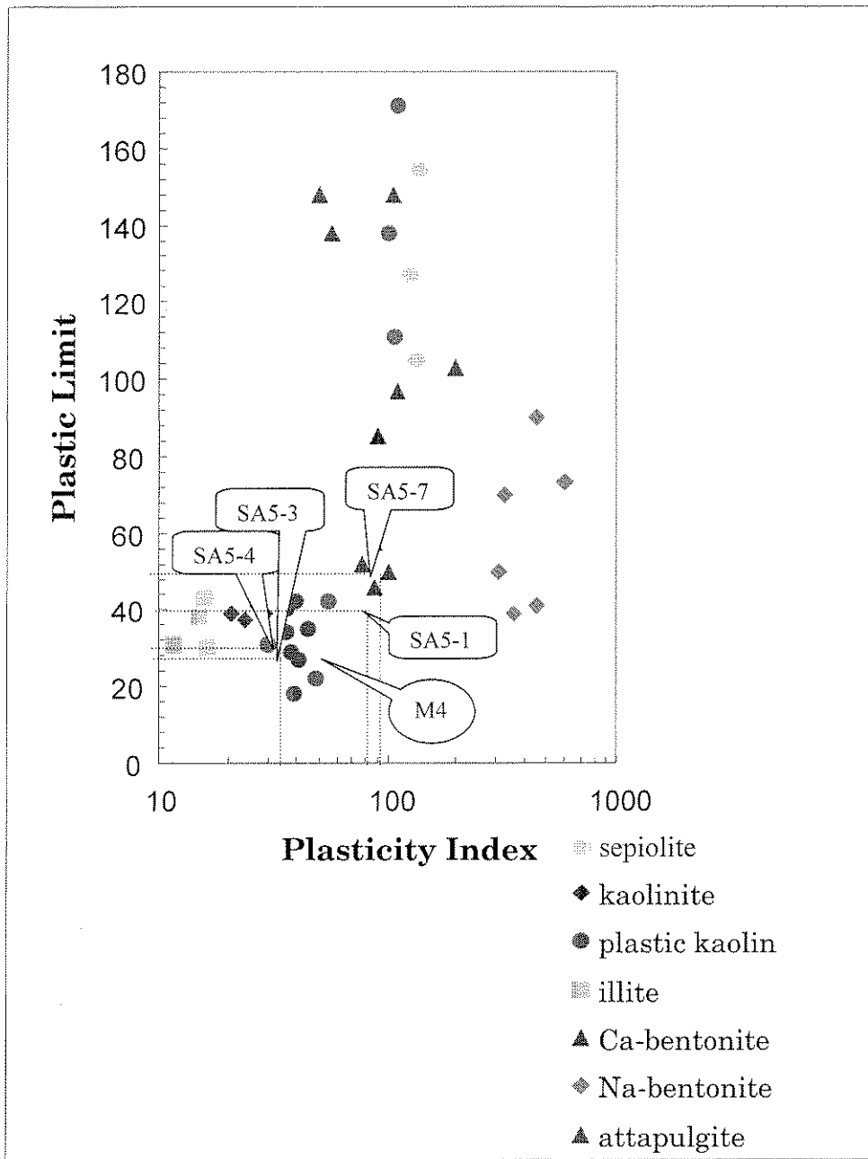
Figure 6. Sabah bentonite plasticity chart
