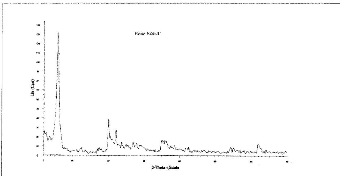
Figure 4. XRD pattern for Andrassy bentonite Sample
