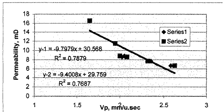
Figure 3. Acoustic Velocity (Vp) Vs Permeability of Rock
