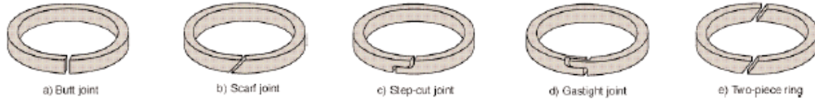
Figure 6 Various types of cut joints for piston rings
