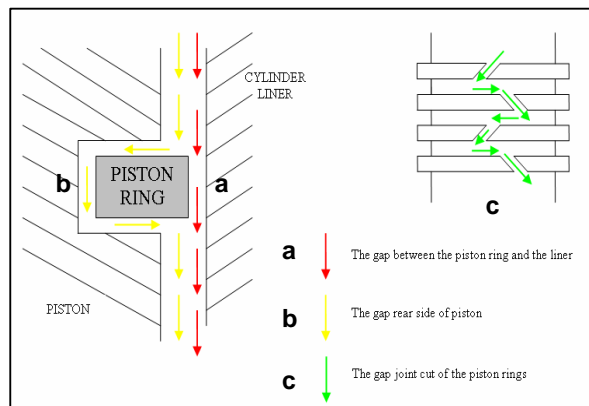
Figure 5. Three possible paths of gas leakage through the rings
