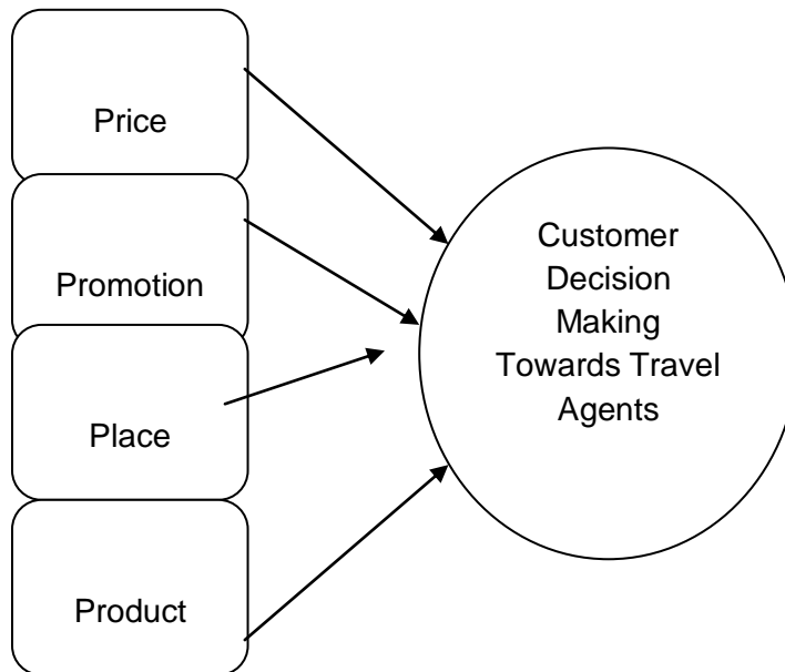
Fig. 1: Conceptual Framework
