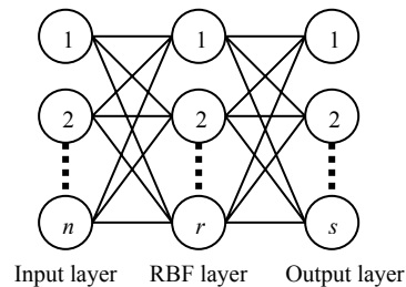
Figure 4 – RBF Neural Network Structure
