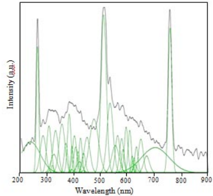
Fig. 4 The emission spectrum of 25Li_2CO_3:25CaO:20B_2O_3:30P_2O_5 with 1 mol% of Mn ions in the excitation of 260 nm.
