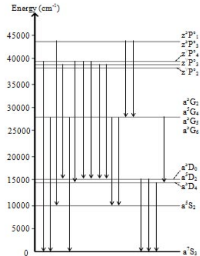
Fig. 5 Energy level diagram of the sample doped Mn ions.
