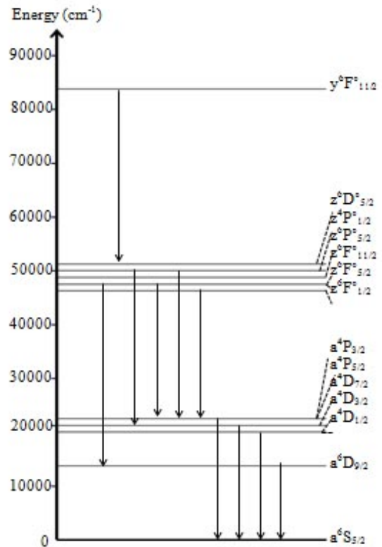
Fig. 3 Energy level diagram of the sample doped Cr ions.
