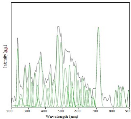
Fig. 5 The emission spectrum of 25Li_2CO_3:25CaO:20B_2O_3:30P_2O_5 with 1 mol% of Fe ions in the excitation of 240 nm.
