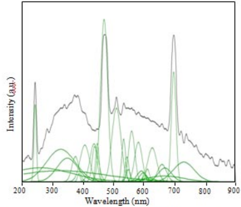
Fig. 2 The emission spectrum of 25Li 2 CO 3 :25CaO:20B 2 O 3 :30P 2 O 5 with 1mol% of Cr ions in the excitation of 240 nm.
