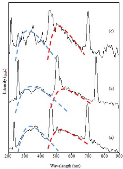
Fig. 1 The emission spectrum of 25Li 2 CO 3 :25CaO:20B 2 O 3 :30P 2 O 5 with (a) 1 mol% of Cr ions, (b) 1 mol% of Mn ions and (c) 1 mol% of Fe ions
