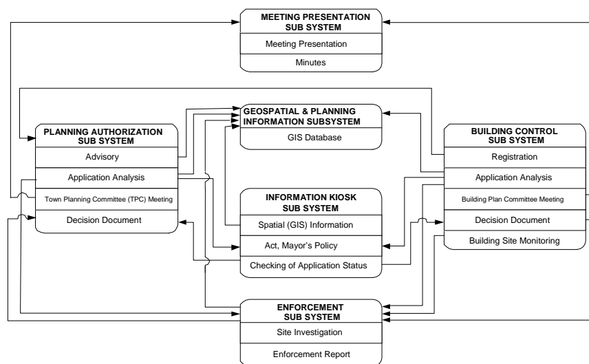
Figure 1: Sub Systems Interaction
