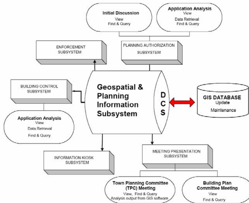
Figure 5: GIS Function in Development Control System Subsystem
