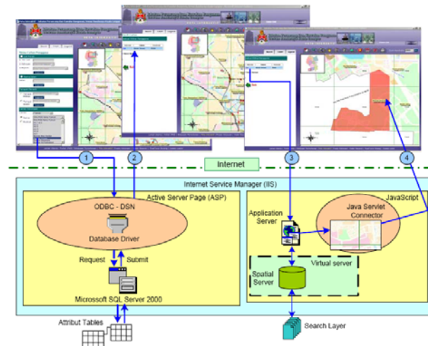
Figure 8: Web GIS Architecture within the Information Kiosk
