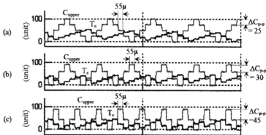
Fig. 13. The zoomed image (zoomed area indicated by '↔') of the waveforms of upper triangular and output of PI controller for (a) DTC-CSF1, (b) DTC-CSF2 and (c) DTC-CSF3, corresponds the results obtained in Fig. 12 (b),(c) and (d). (Time scale: 1 ms/div.)
