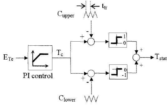
Fig. 4. Constant frequency torque controller (CFTC).
