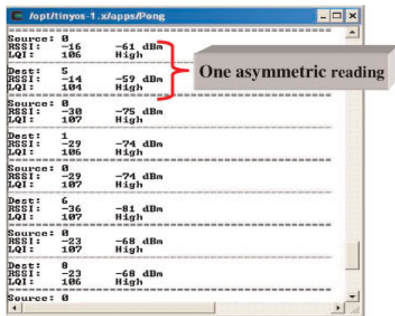
Figure 10. Asymmetric signal strength reading.
