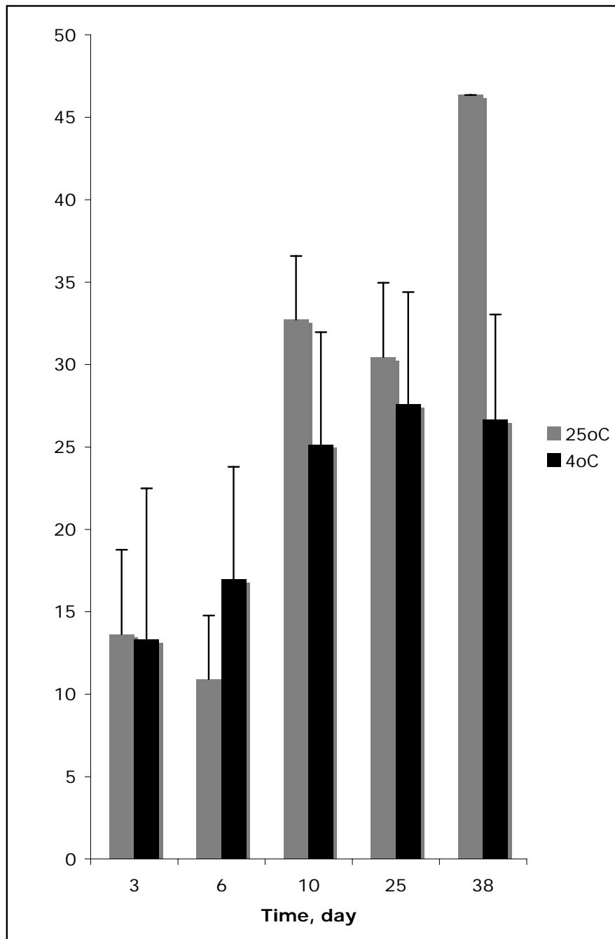
Figure 4.2 Comparison of apparent enzyme activity for PVA-GOD membranes immobilized at 25°C and 4°C.
