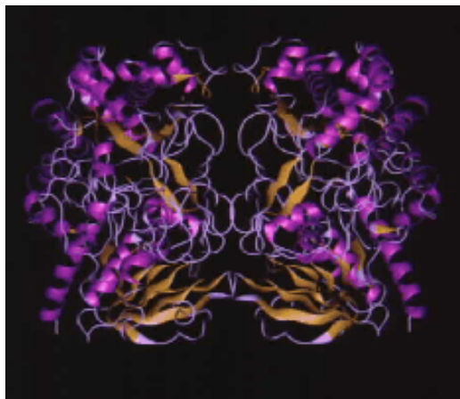
Figure 2.1 Overall topology of Glucose oxidase.
