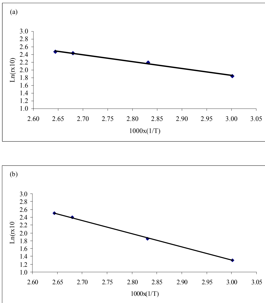
Figure 4.19. Plots of logarithmic crosslinking rates as a function of reciprocal absolute temperature for the 1-phr silane-grafted HDPE samples with (a) 0.5 \pm 0.05 mm and (b) 1.0 \pm 0.05 mm thickness.
