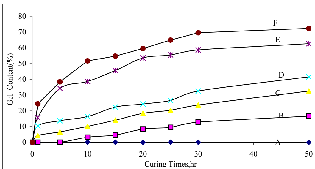
Figure 4.11: Plots of the gel contents of the 1.8-phr silane-grafted HDPE bottle samples with 1.00\pm 0.05 mm in thickness as a function of crosslinking time at (A) 30^{\circ}\text{C} , (B) 60^{\circ}\text{C} , (C) 80^{\circ}\text{C} , (D) 95^{\circ}\text{C} , (E) 100^{\circ}\text{C} , and (F) stream (1bar).
