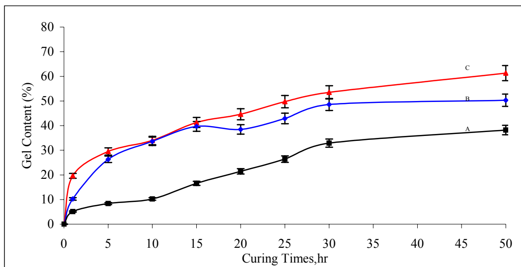
Figure 4.13: Plots of the gel contents of the (A) 1.6-phr, (B) 1.8-phr, and (C) 2.0-phr silane-grafted HDPE samples with 0.5 \pm 0.05 mm in thickness as a function of crosslinking time at 80°C.
