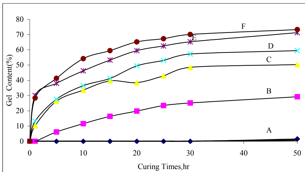
Figure 4.10: Plots of the gel contents of the 1.8-phr silane-grafted HDPE bottle samples with 0.5\pm 0.05 mm in thickness as a function of crosslinking time at (A) 30^{\circ}\text{C} , (B) 60^{\circ}\text{C} , (C) 80^{\circ}\text{C} , (D) 95^{\circ}\text{C} , (E) 100^{\circ}\text{C} , and (F) stream (1bar).
