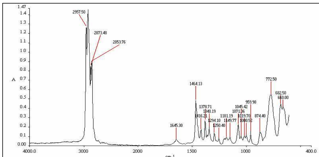
Figure 4.21: FTIR spectrum of Bis (tributyltin) oxide from the mechanical fine additive residue.
