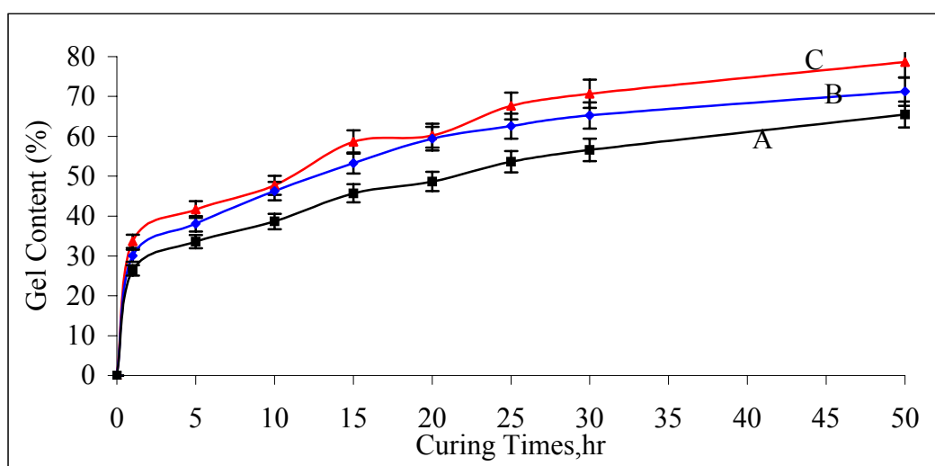
Figure 4.14: Plots of the gel contents of the (A) 1.6-phr, (B) 1.8-phr, and (C) 2.0-phr silane-grafted HDPE samples with 0.5 \pm 0.05 mm in thickness as a function of crosslinking time at 100°C.
