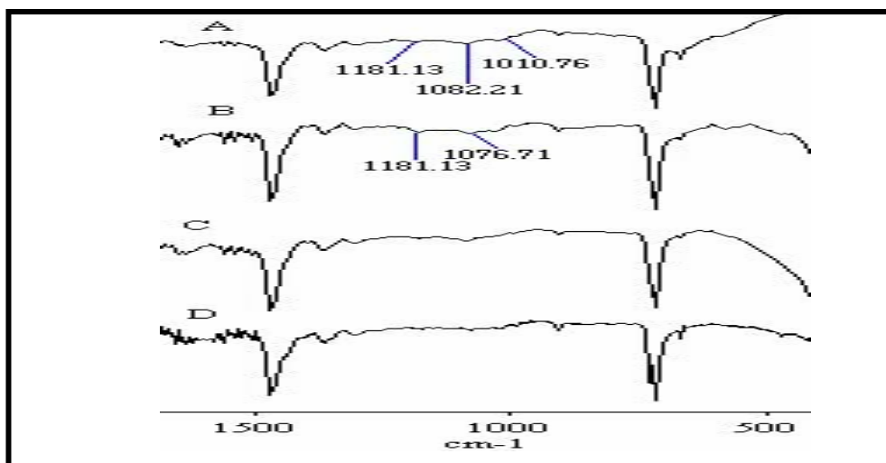
Figure 4.24: FTIR spectra of crosslinked HDPE containing 2.0 phr VTMO and 0.01 phr DBTL with various concentration of DCP (A) 0.5 phr, (B) 0.4 phr, (C) 0.2 phr and (D) 0.1 phr, followed by crosslinking with boiled water for 5 hours.
