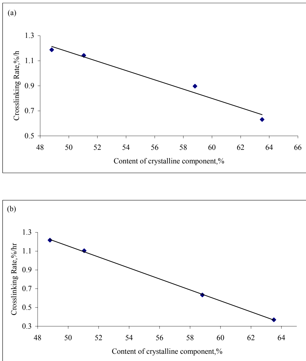
Figure 4.17: Plots of the crosslinking rates as a function of the content of crystalline component for the 1.8-phr silane-grafted HDPE samples with (a) 0.5 \pm 0.05 mm and (b) 1.0 \pm 0.05 mm thickness
