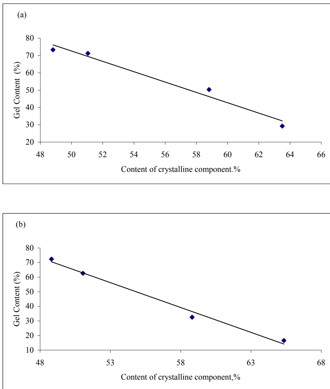
Figure 4.18. Plots of the gel contents as a function of the content of crystalline component for the 1.8-phr silane-grafted HDPE samples with (a) 0.5 \pm 0.05 mm and (b) 1.0 \pm 0.05 mm thickness.
