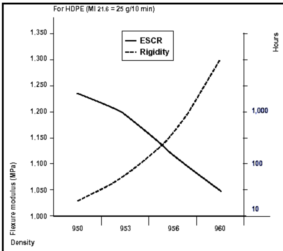
Figure 2.10: Evolution of stress cracking resistance and rigidity relative to density [57, 58].
