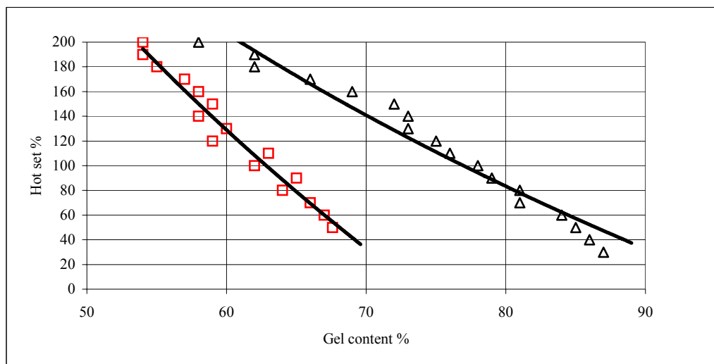
Figure 4.26 : The relationship on the hot set test against its gel content.Δ- Silane polyfunctional crosslinked PE, □- peroxide initiator crosslinked PE.
